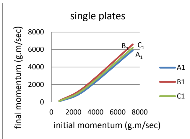
Fig.2. Relationship between initial momentum and final Bullet velocity single plate
