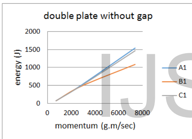
Fig. 6. Relationship between the initial momentum and the absorbed energy, double plate without gap
