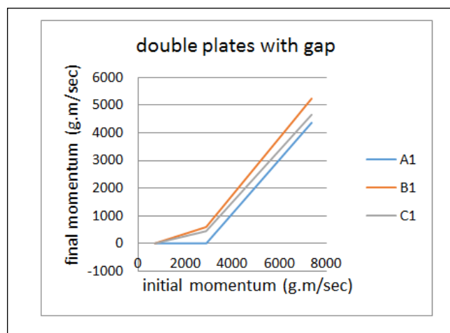
Fig.4. Relationship between initial momentum and final Bullet Velocity doubles plate with gab
